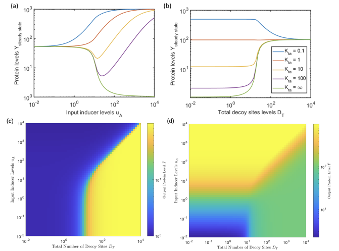
Fig. 7. Paradoxical effect in steady-state levels of the output protein portrayed for varying the levels of (a) activator input levels ( u_A for D_T = 20 ) and (b) total decoy sites ( D_T for u_A = 10 ) in the system. Two parameter bifurcation plots between u_A and D_T showing the existence of the paradoxical effects for (c) K_{ta} \rightarrow \infty and its absence for (d) K_{ta} = 0.1 . The parameter values used for the simulation are: K_{tr} = 0.1, K_{dr} = 0.1, K_{da} = 0.1, T_T = 1, R_T = 10, \kappa = 1000, \beta = 100 , and \gamma = 1 .
