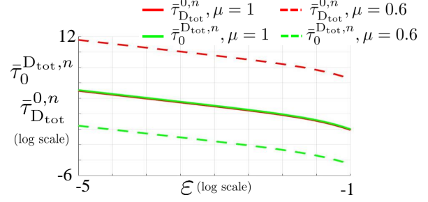
Fig. 5: Effect of \varepsilon and \mu on the time to memory loss. Graph of the analytical expressions of the normalized time to memory loss for both the repressed and active chromatin states as a function of \varepsilon for different \mu values. The y axis is in log scale and show \bar{\tau}_{D_{\text{tot}}}^{0,n} and \bar{\tau}_0^{D_{\text{tot},n}} , that are the values of \tau_{D_{\text{tot}}}^0 and \tau_0^{D_{\text{tot}}} divided by their corresponding values for \varepsilon = 0.1 and \mu = 1 . The formulas of the \bar{\tau}_{D_{\text{tot}}}^0 and \bar{\tau}_0^{D_{\text{tot}}} are given in (28) and (30), respectively. The parameter values considered are k_{W0}^A = k_{W0}^R = 5h^{-1} , k_W^A = k_W^R = 0 , k_M^A/\Omega = k_M^R/\Omega = 1h^{-1} , u_{A0} = u_{R0} = 0.1 , u_A = u_R = 0 , \alpha = 1 , b = 1 , \varepsilon' = 0.1 , \varepsilon = (10^{-5}, 10^{-1}) , \mu = 0.6, 1 , D_{\text{tot}} = 50 .
