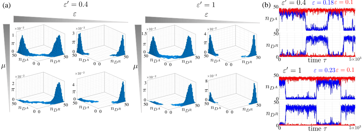
Fig. 6: Stochastic simulations of the histone modification circuit in Fig. 1(a) using SSA. (a) The stationary distribution for the histone modification circuit whose reactions are listed in Fig. 1(a). The parameter values are in Table II. In particular, in the left-side plots \varepsilon = 0.18, 0.1 , \mu = 1, 0.8 and \varepsilon' = 0.4 and in the right-side plots \varepsilon = 0.23, 0.1 , \mu = 1, 0.8 and \varepsilon' = 1 . In all plots n_{DA} and n_{DR} represent the number of nucleosomes with active histone marks and repressive histone marks, respectively. (b) Time trajectories of n_{DA} and n_{DR} starting from the fully active state n_{DA} = 50, n_{DR} = 0 for different values of \varepsilon and \varepsilon' . The time is normalized ( \tau = t \frac{k_{w0}^A}{\Omega} D_{\text{tot}} , with \Omega the reaction volume) and the parameter values are in Table II.
